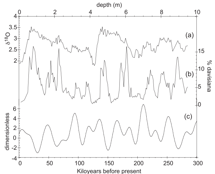
FIGURE 4: Core RC11-120, drilled through 953 cm of sediment in the Indian Ocean (43°31'S, 79°52'E) from a water depth of 3193 m, and sampled at 5 cm intervals. (a) G. bulloides δ 18 O; (b) C. davisiana abundance with core depth (top horizontal axis). The two data sets do not share the same depth points. (c) ETP signal over 0–300,000 y before present (bottom horizontal axis, according to the La2004 model computed with Analysieries ; link in Supplemental Materials).
